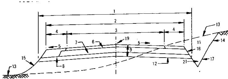
PAVED ROAD SECTION
