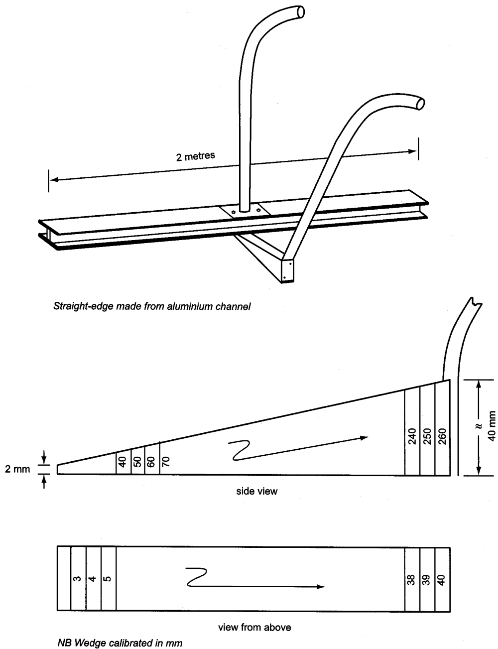
Figure 4.5 Straight edge and calibrated wedge
