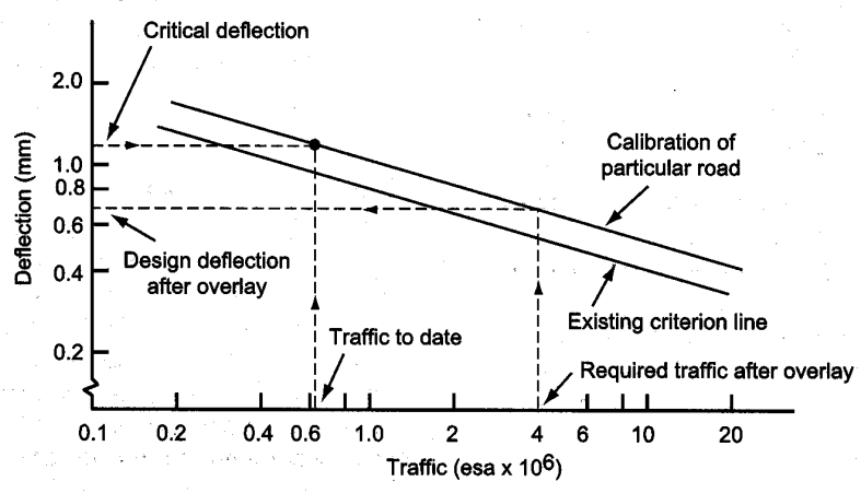
Figure 9.1 Diagrammatic calibration of deflection life criterion line (after NITRR, 1983)
