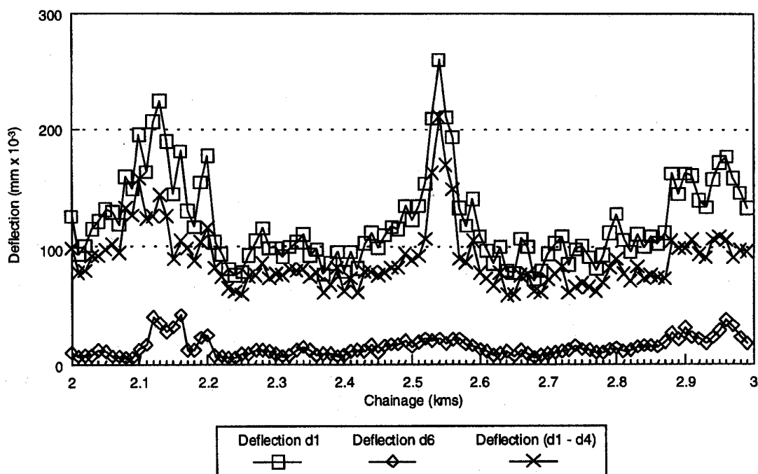
Figure 7.3 FWD deflection profile
