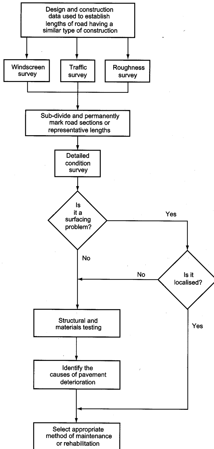
Figure 2.1 Road pavement evaluation and rehabilitation procedure
