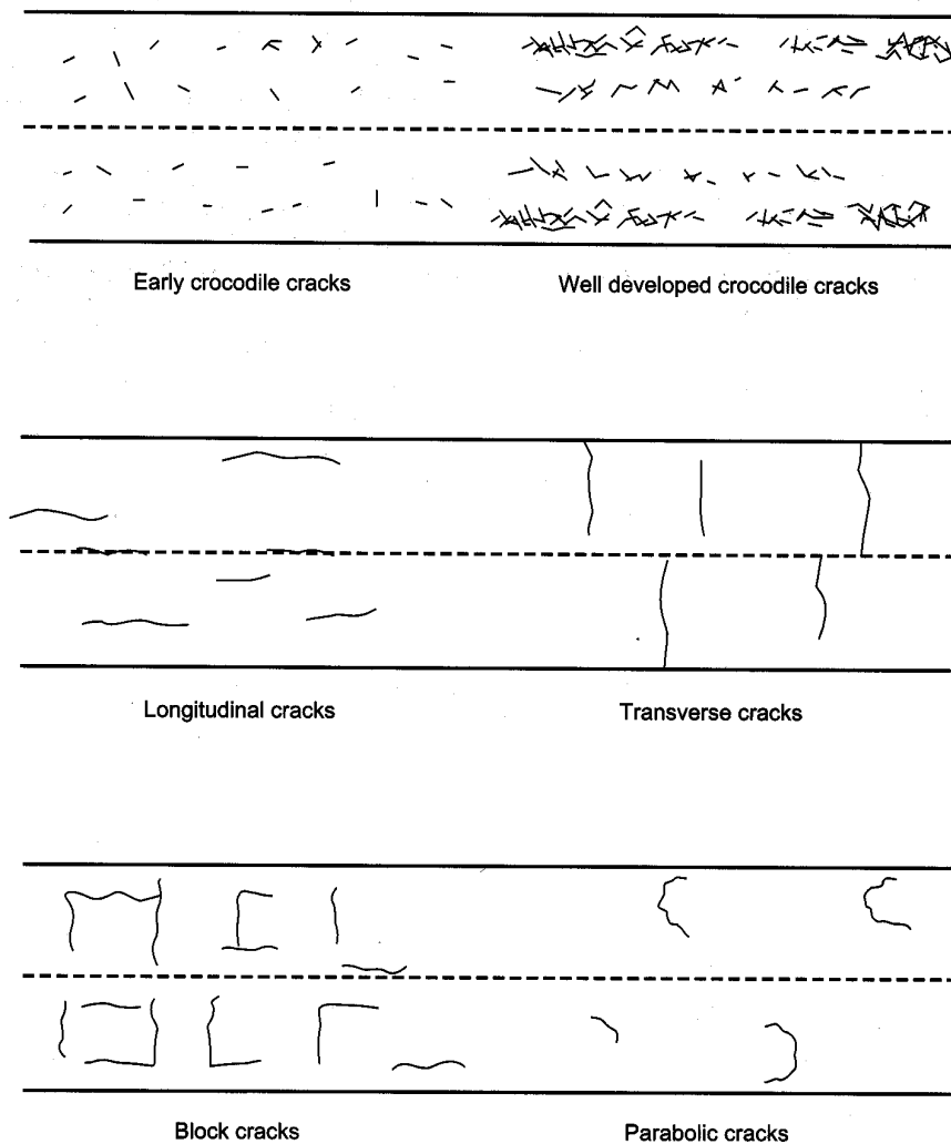
Figure 4.3 Types of cracking
