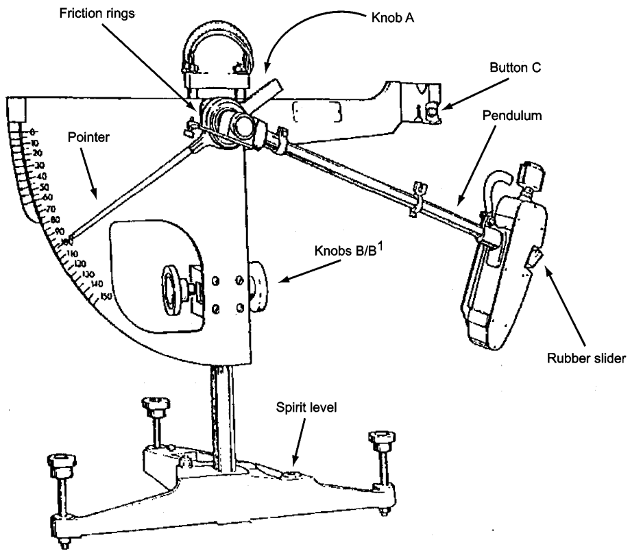
Figure 11 Portable skid-resistance tester
