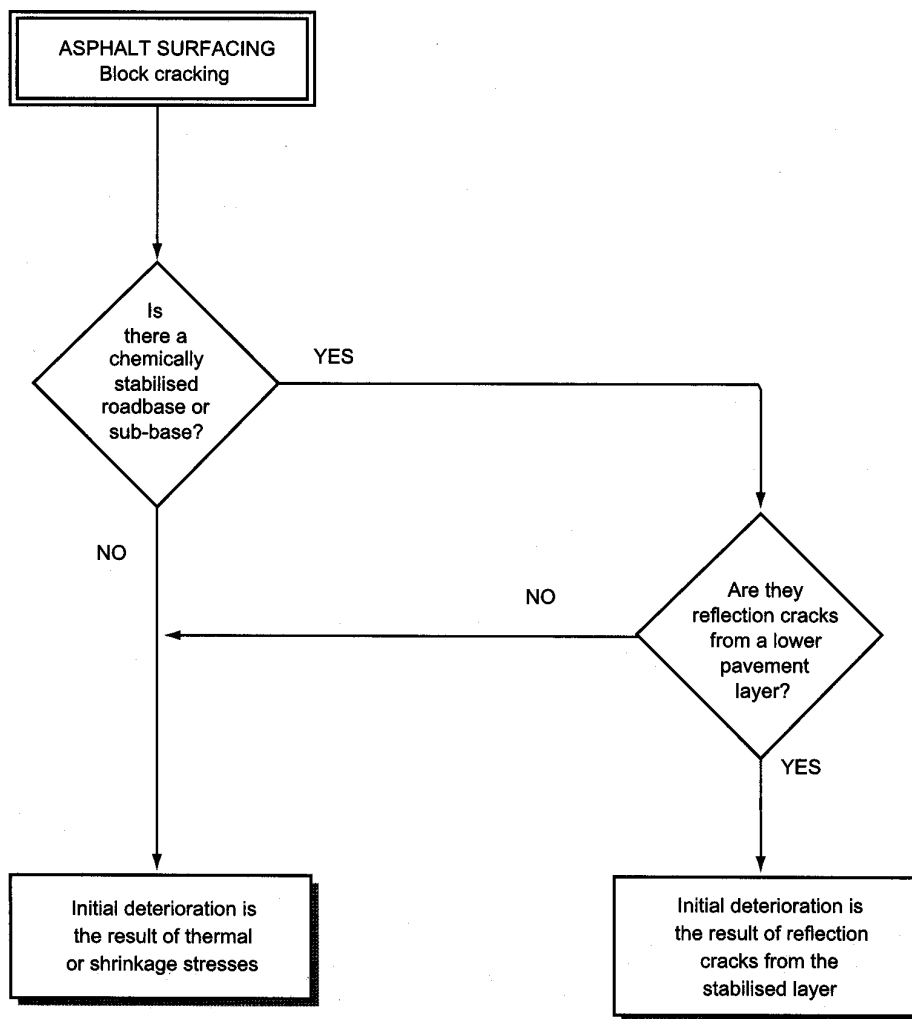
Figure 8.8 Initial deterioration - Block cracking in asphalt surfacing
