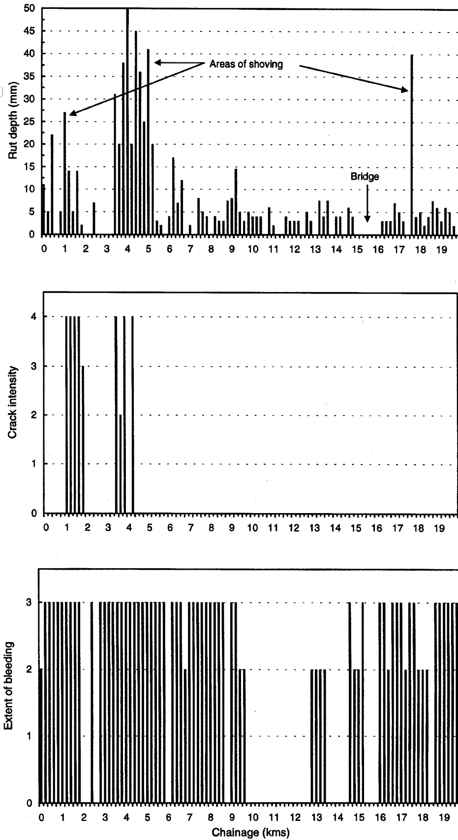
Figure 6.2 Illustration of performance charts
