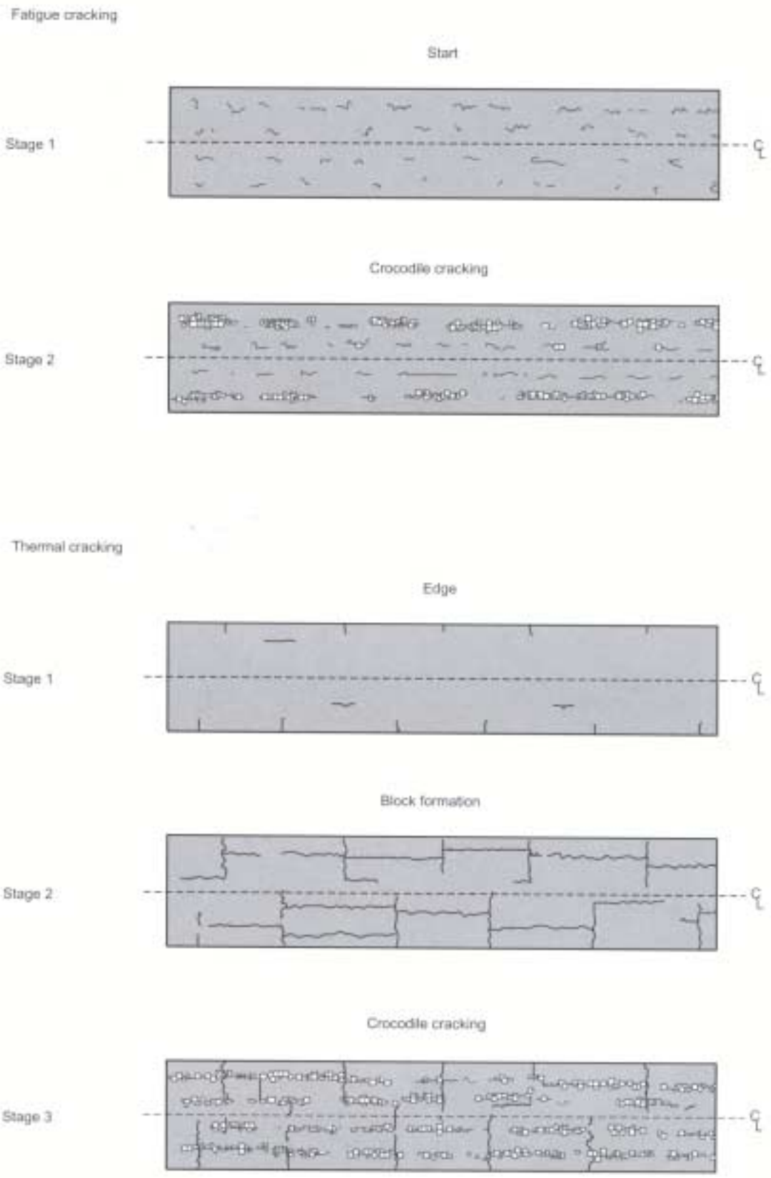
Figure 8.9 Crack development patterns in bituminous surfacings (after Dickinson, 1984)
