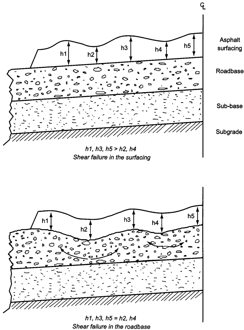
Figure 4.6 Transverse core profile to investigate rutting
