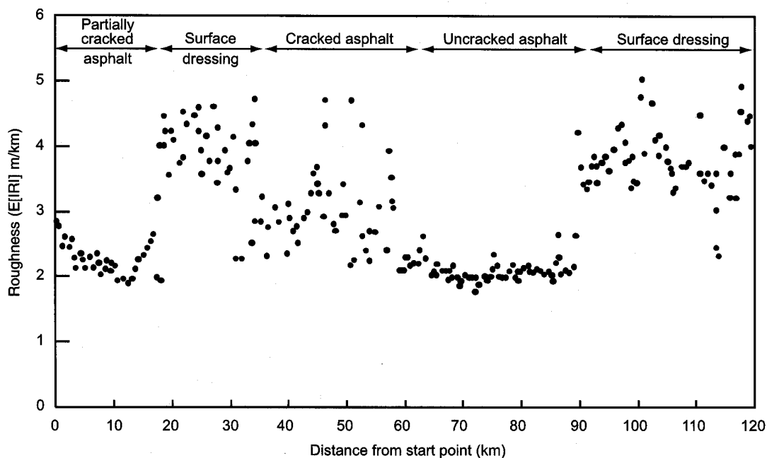
Figure B4 Road roughness profile
