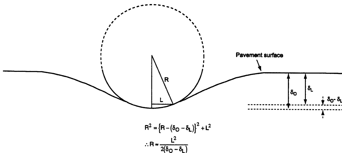
Figure 7.2 Computation of radius of curvature
