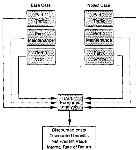
FIGURE 1 Program structure.
