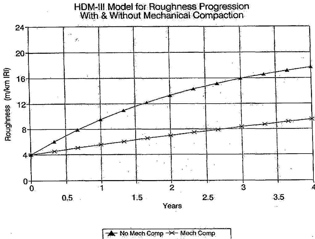
Figure 5: Modelled Roughness Progression with and without Mechanical Compaction
